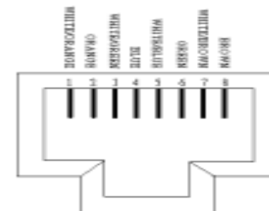
RJ45 PIN AND CABLE COLORS
